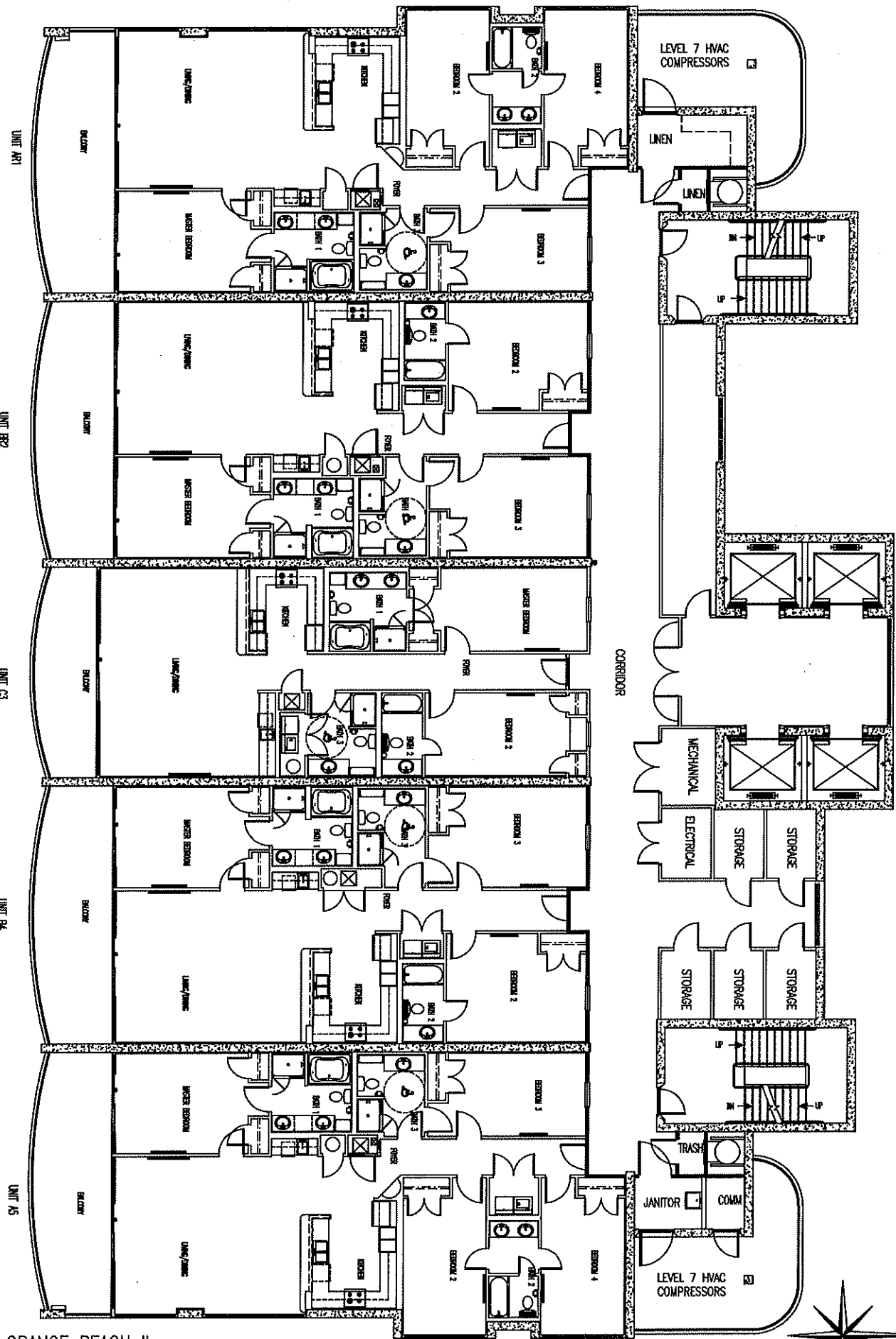
PHOENIX ORANGE BEACH II 7TH THRU 27TH FLOOR PLAN (NO 13TH FLOOR)
